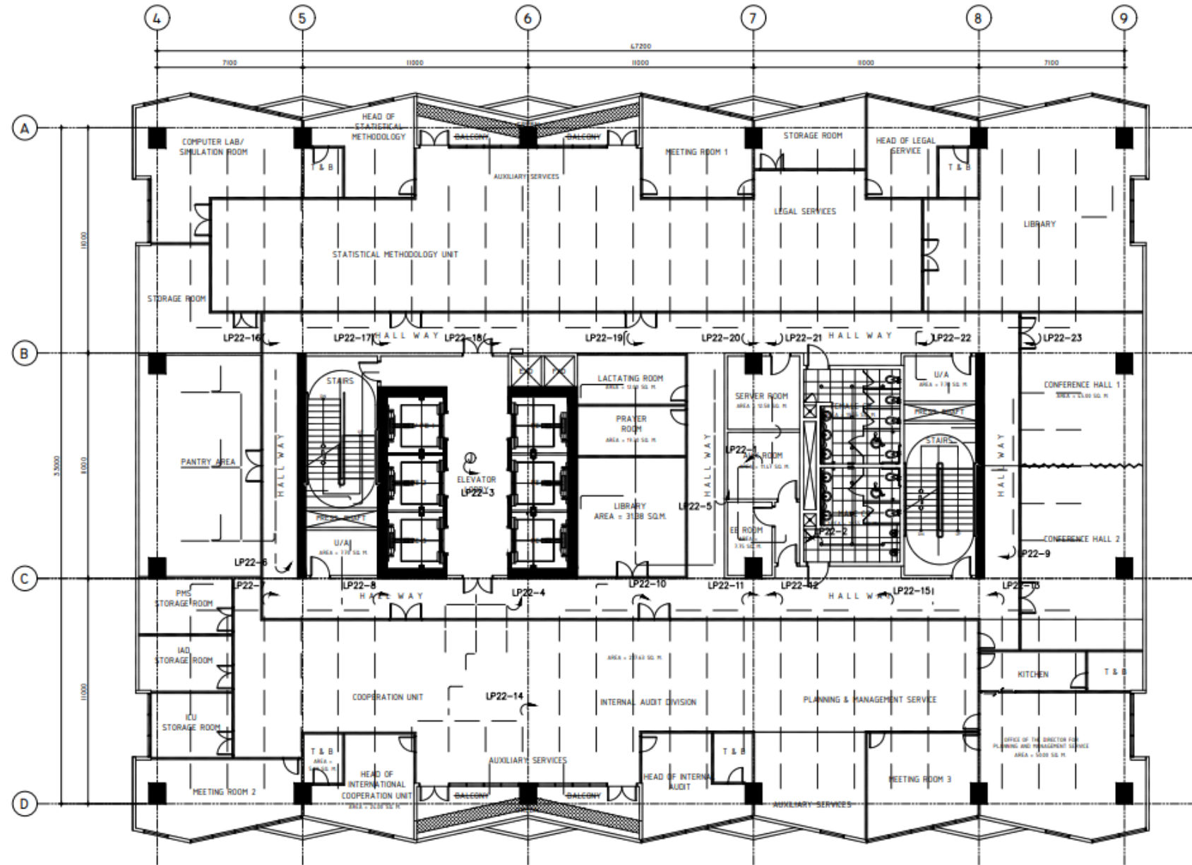
○ LIGHTING LAYOUT SCALE 1:200 MTS
