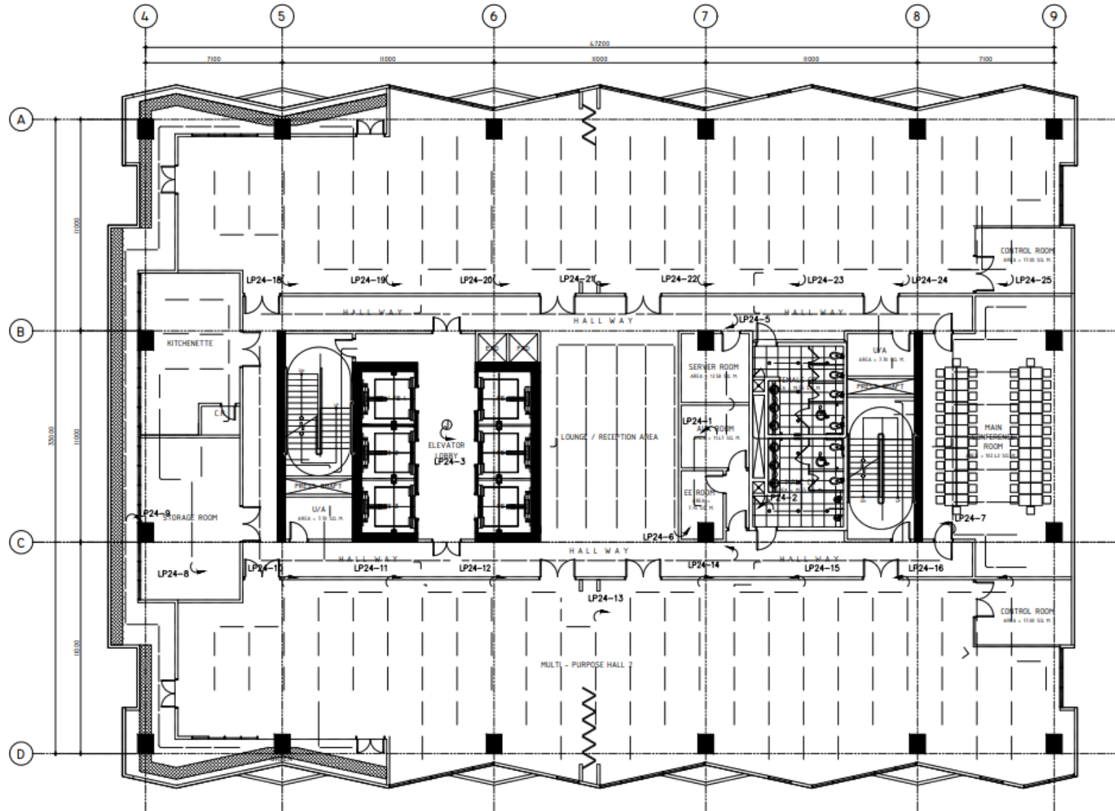
LIGHTING LAYOUT SCALE 1:200 MTS
