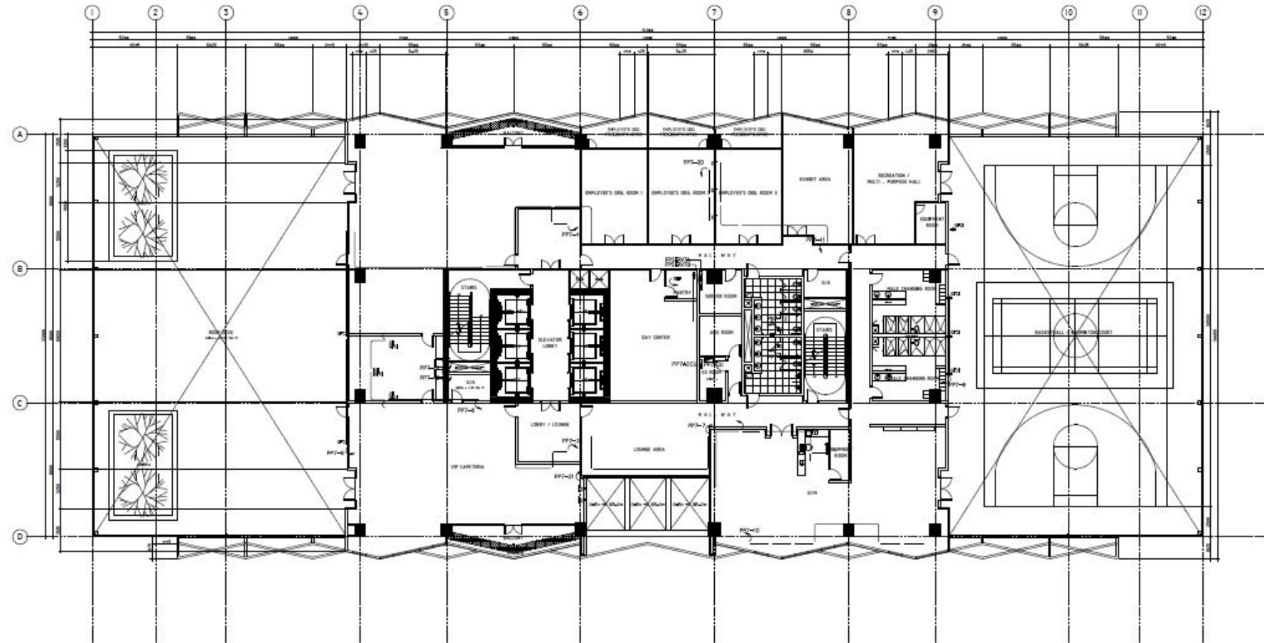
POWER LAYOUT SCALE: 1:300 MTS
