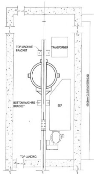
ELEVATION IN HOISTWAY LOOKING AT MACHINE
