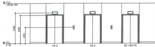
ELEVATOR DOOR ELEVATIONS
