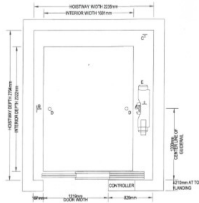
HOISTWAY PLAN VIEW
