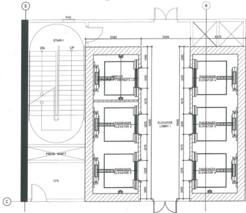
GROUND FLOOR PLAN (BLOW-UP 1)
