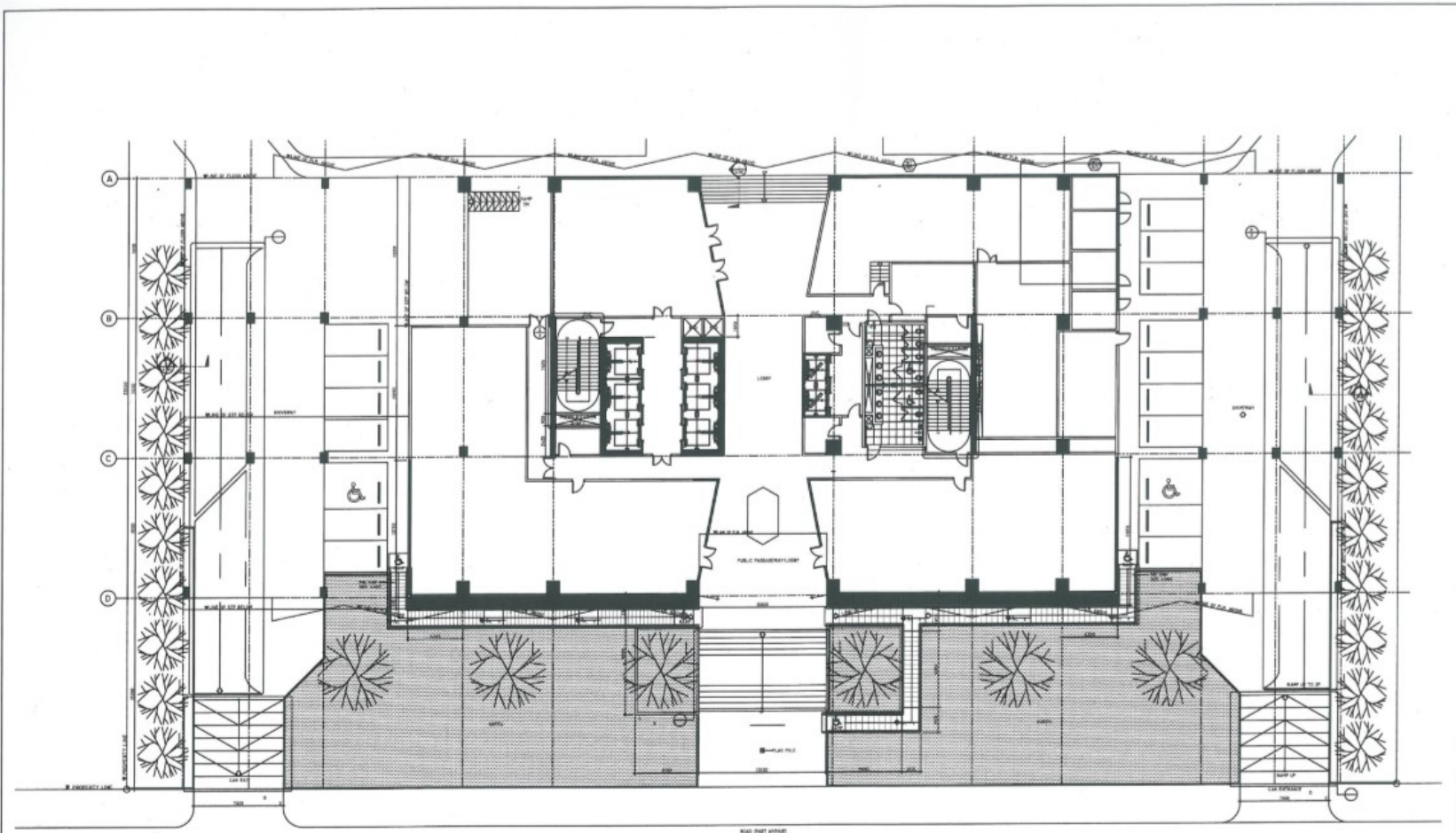
GROUND FLOOR PLAN SCALE: 1:300 M
