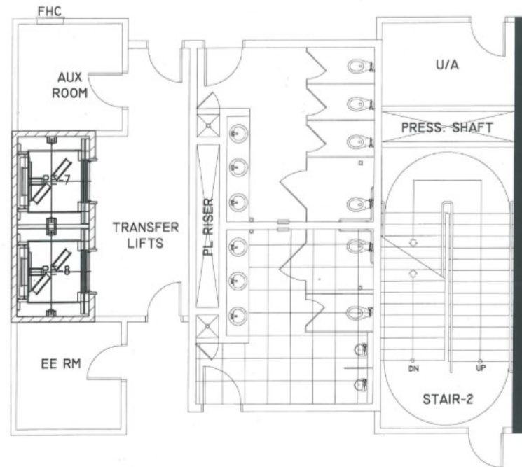
GROUND FLOOR PLAN (BLOW-UP 2)
