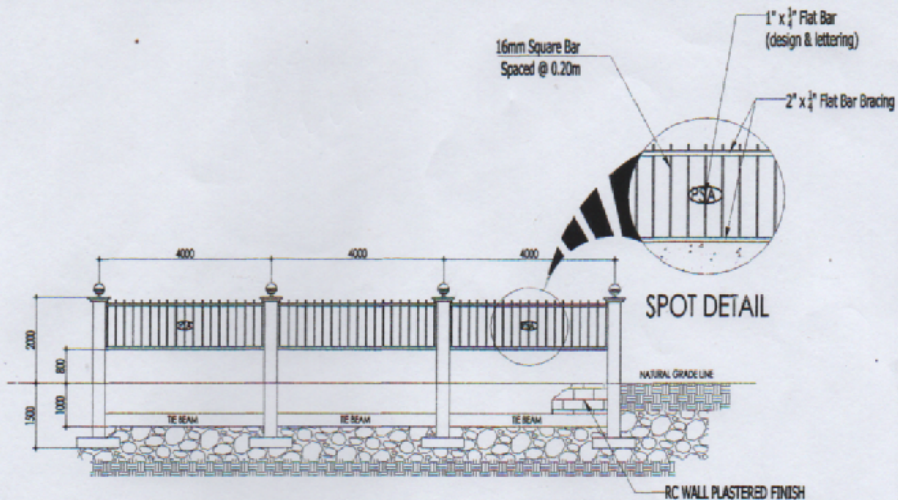
2 TYPICAL FENCE DETAIL SCALE NOTS
