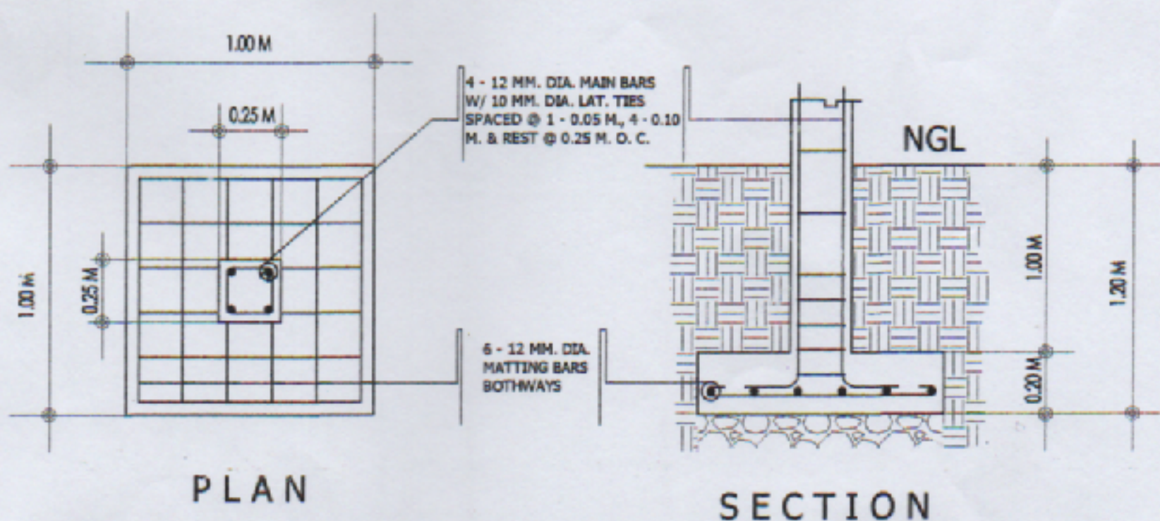
4 COLUMN/FOOTING DETAIL SCALE NOTS
