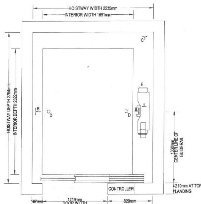
HOISTWAY PLAN VIEW
