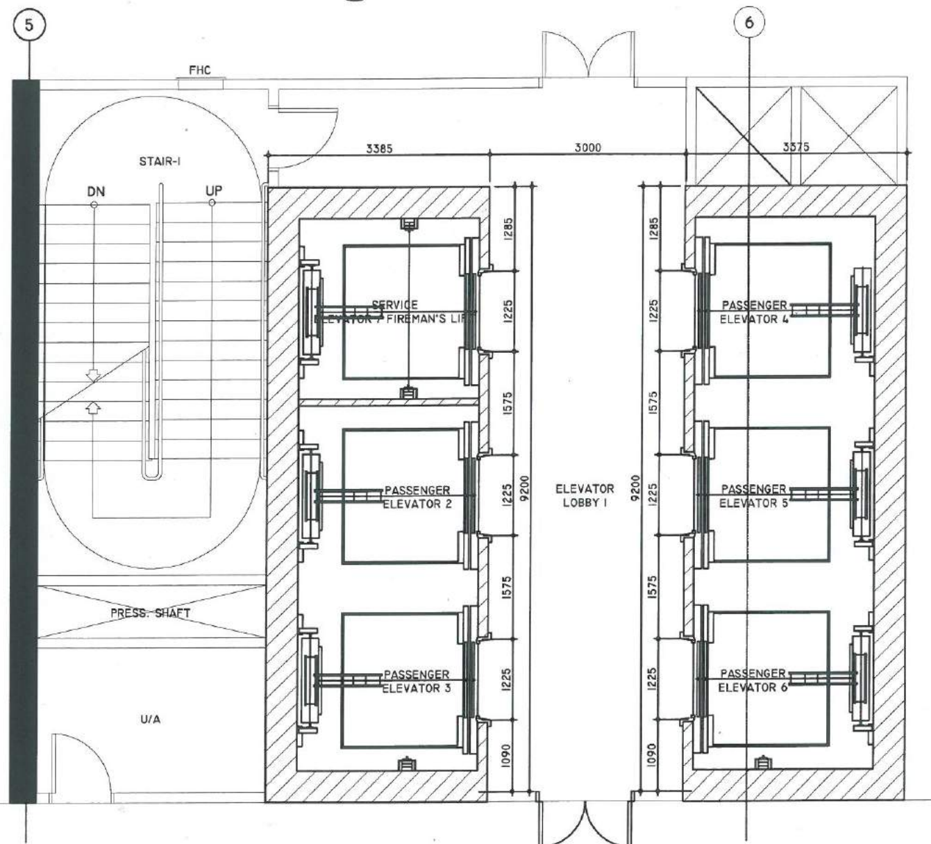
GROUND FLOOR PLAN (BLOW-UP 1)
