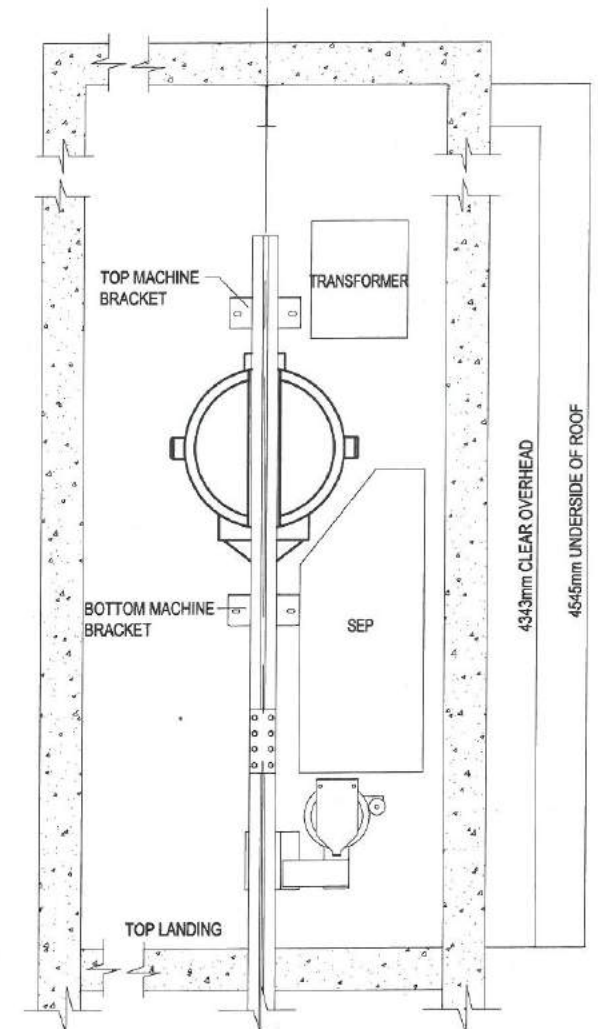
ELEVATION IN HOISTWAY LOOKING AT MACHINE
