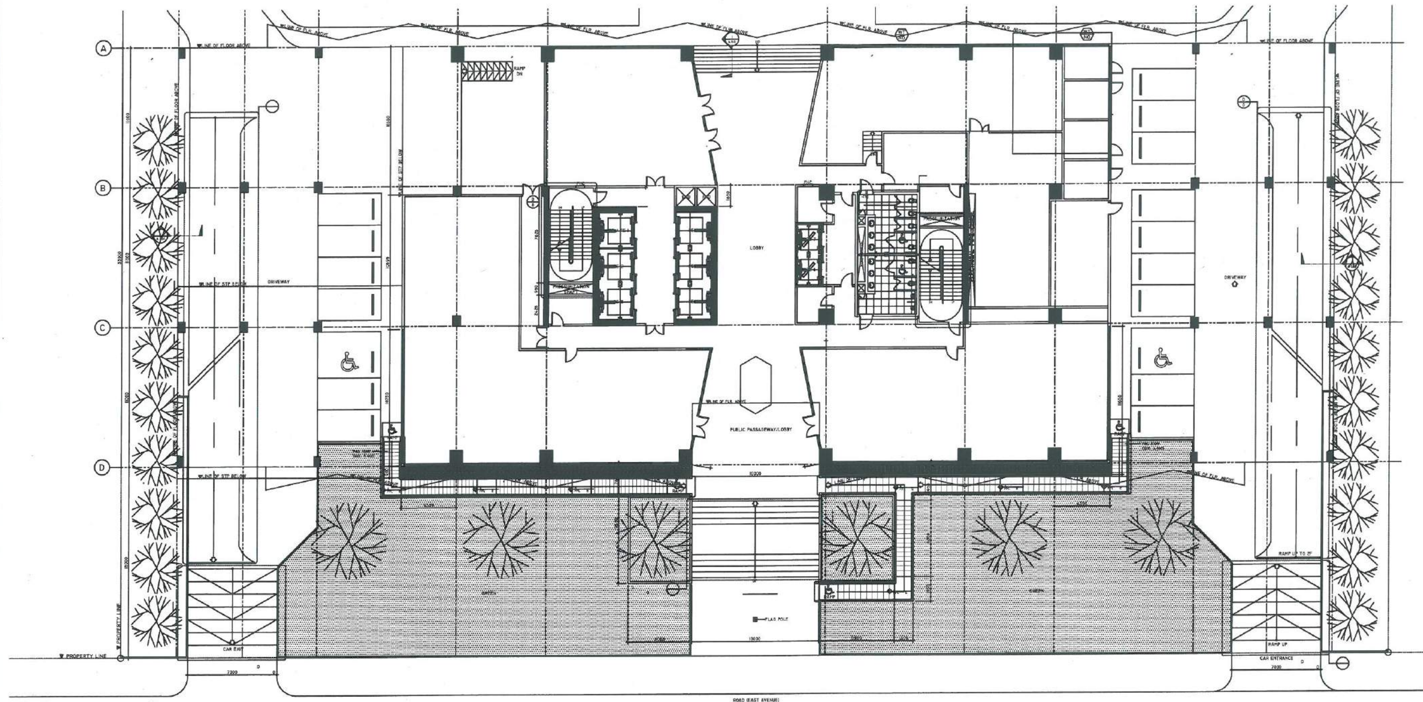
GROUND FLOOR PLAN SCALE: 1:300 M
