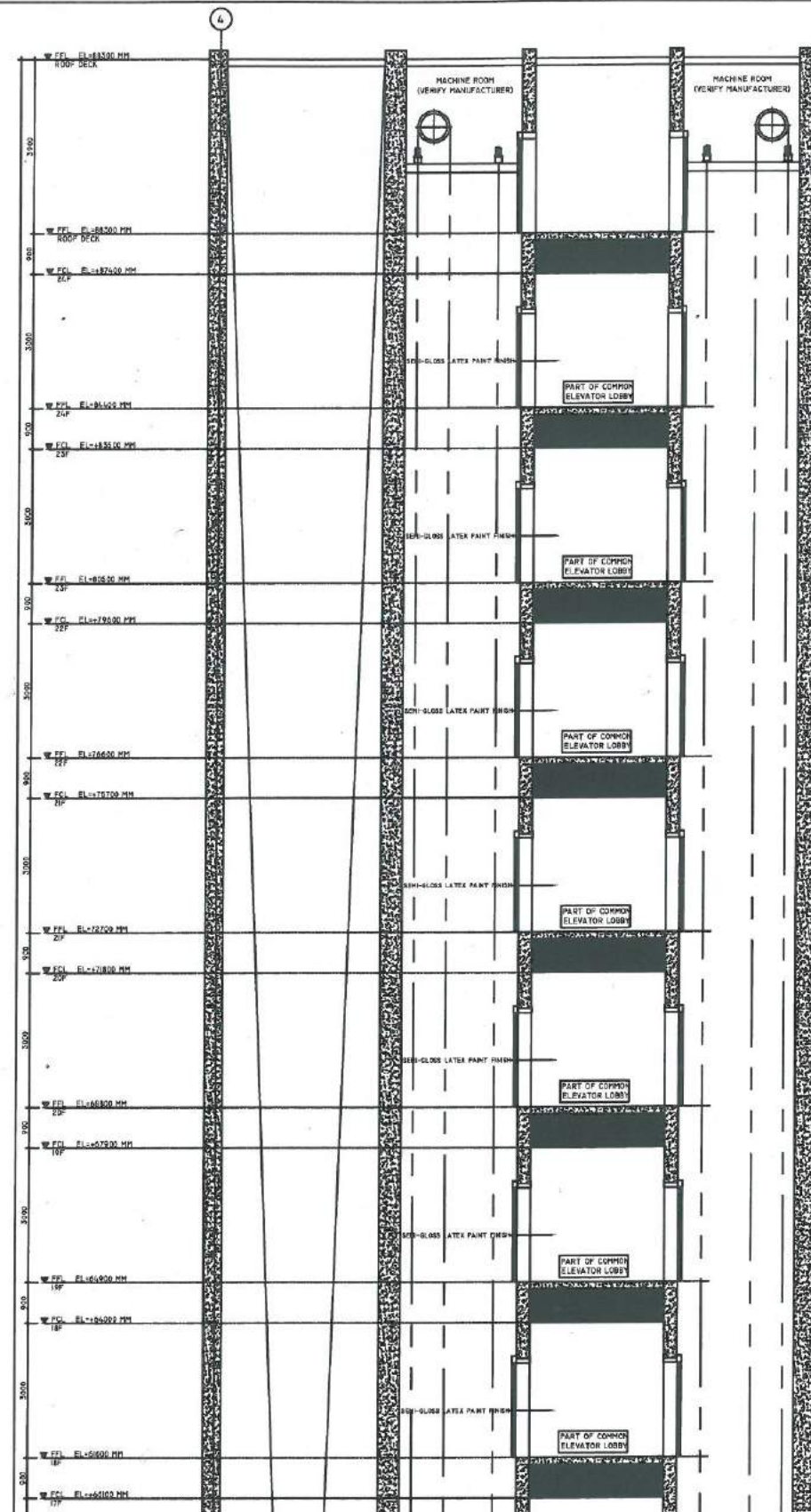
CROSS SECTION OF ELEVATOR SHAFT (OFFICE BUILDING)
