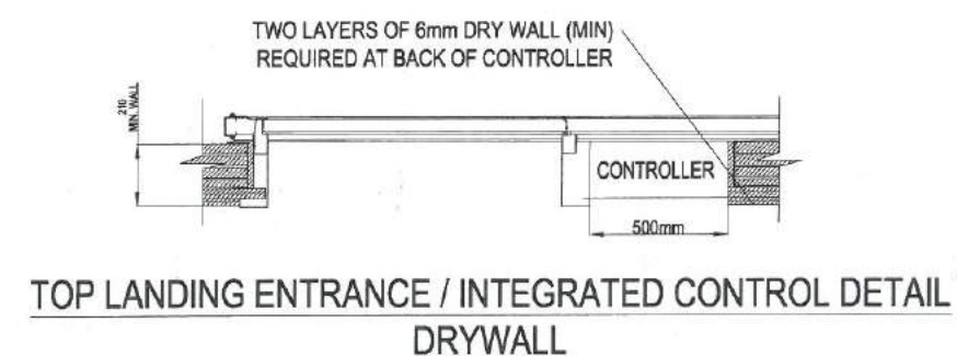
TOP LANDING ENTRANCE DETAILS
