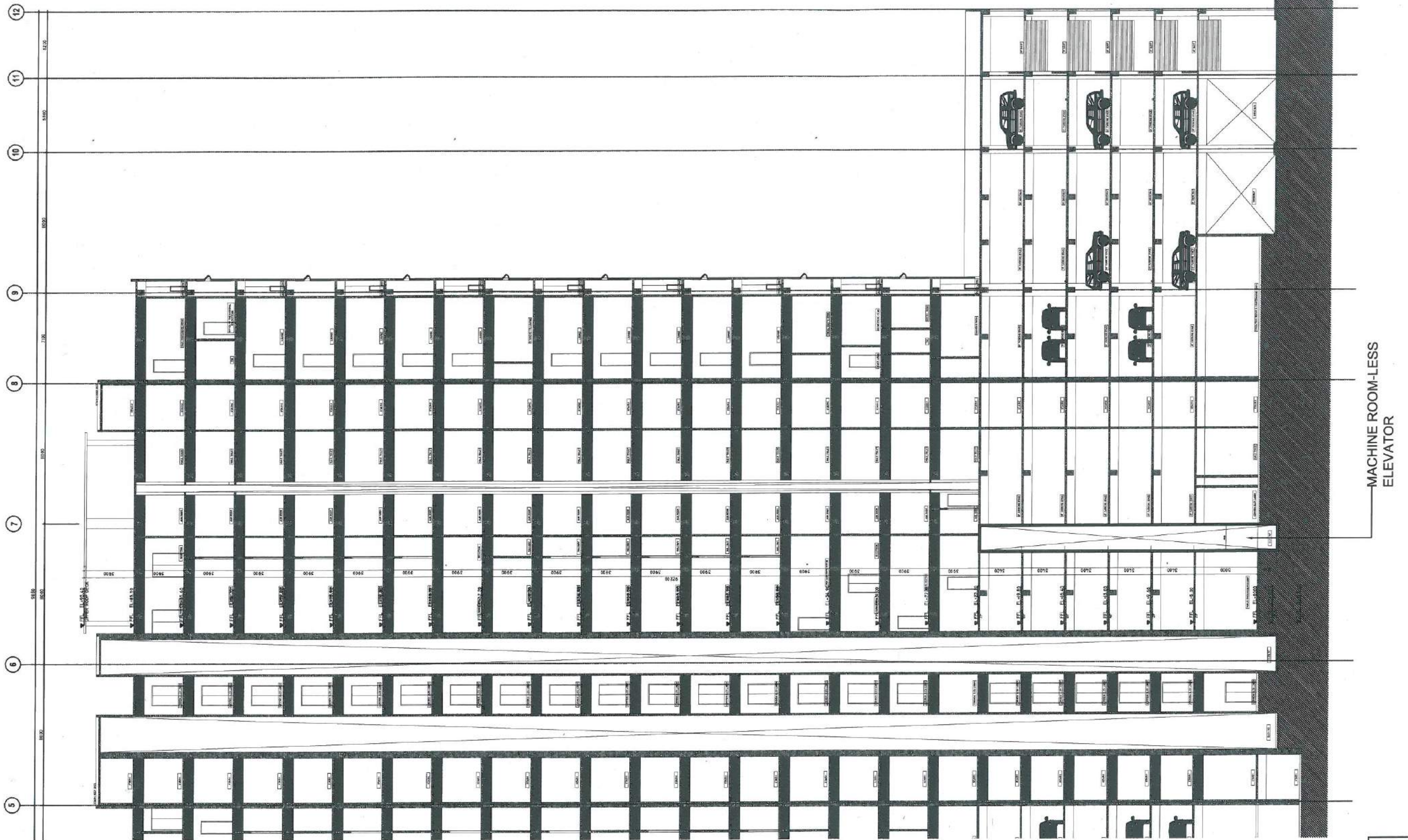
CROSS SECTION OF ELEVATOR SHAFT (PARKING BUILDING)
