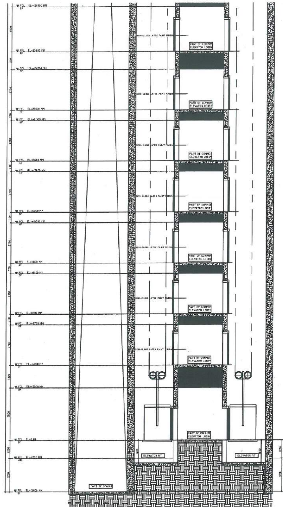
CROSS SECTION OF ELEVATOR SHAFT (OFFICE BUILDING) SCALE: 1:150 M
