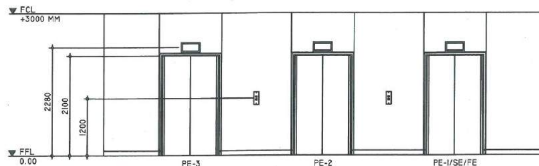
ELEVATOR DOOR ELEVATIONS
