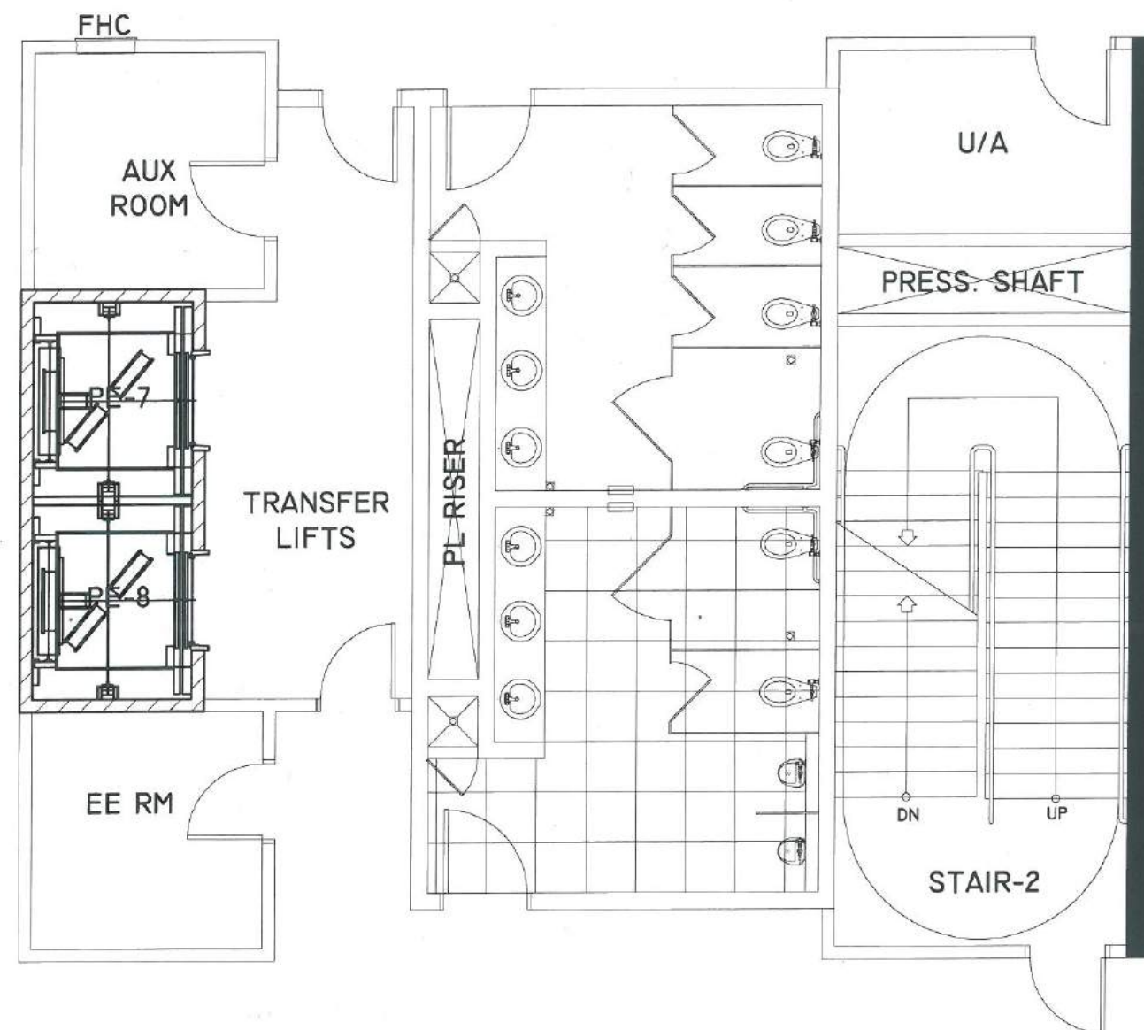
GROUND FLOOR PLAN (BLOW-UP 2)
