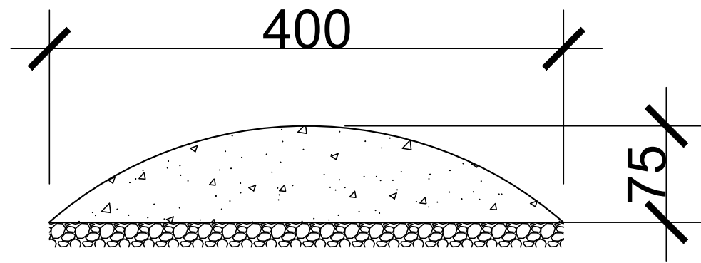
SPEED HUMPS PLAN
