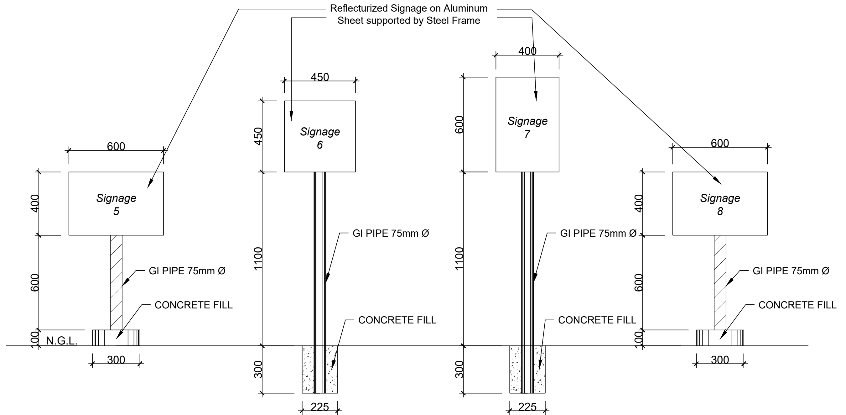
TRAFFIC SIGNAGES (ELEVATION) SCALE: 1:30 M
