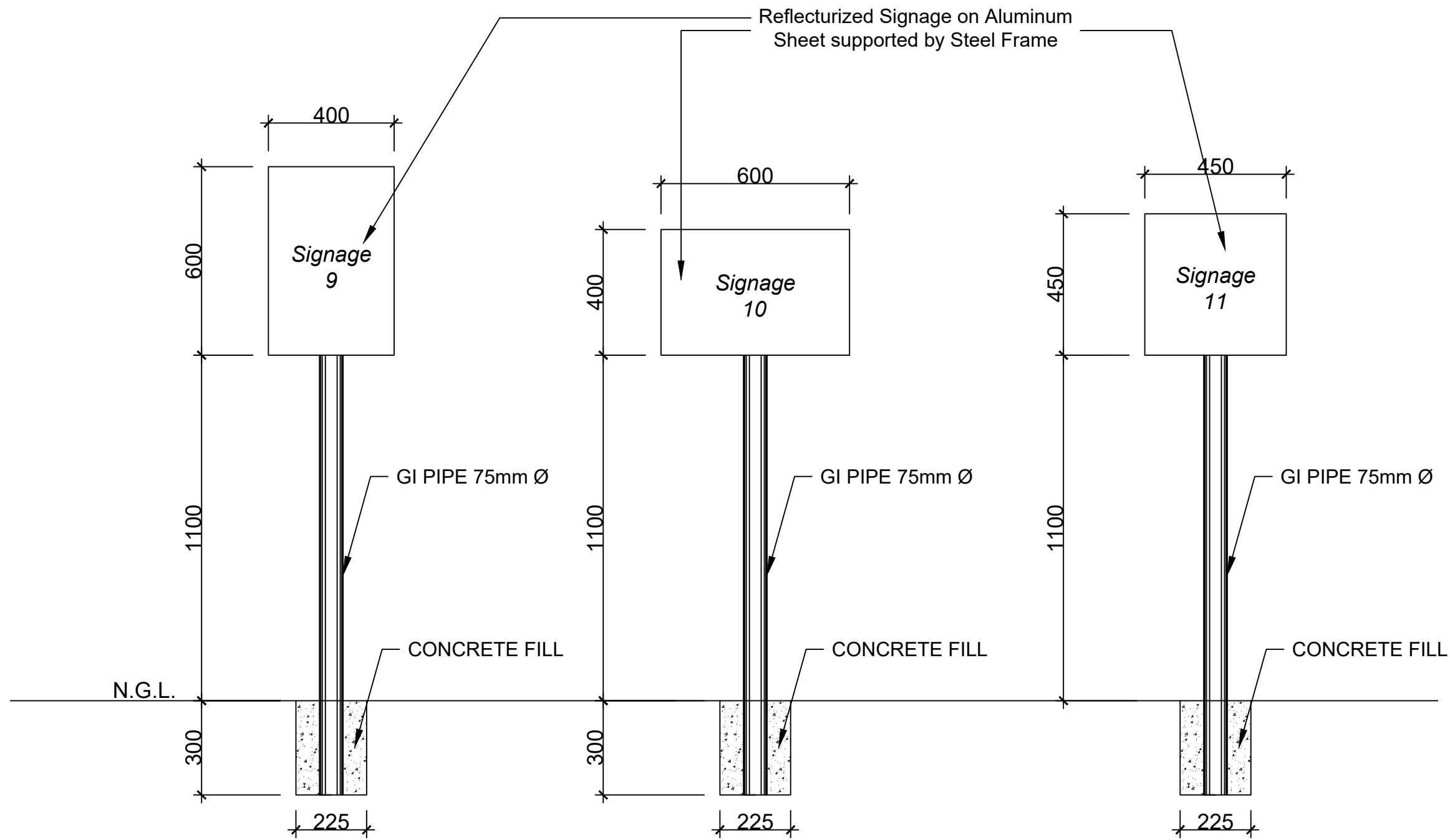
TRAFFIC SIGNAGES (ELEVATION) SCALE: 1:30 M
