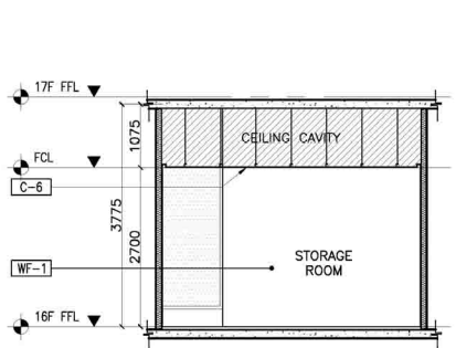
3 16F LPSD & FSD STORAGE ROOM (RIGHT) SECTION THRU "C" A-910F SCALE: 1:50M
