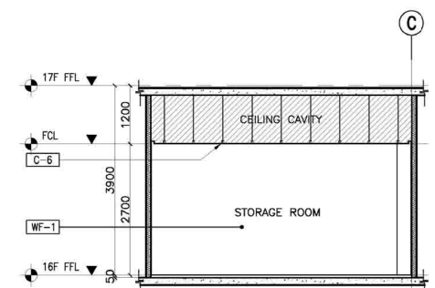
6 16F LPSD & FSD STORAGE ROOM (LEFT) SECTION THRU "B" A-910F SCALE: 1:50M
