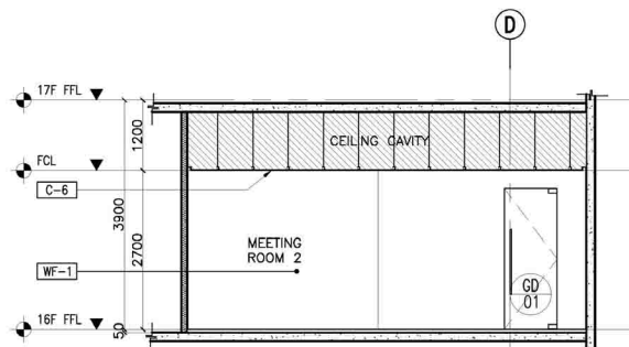
12 16F LPSD & FSD MEETING ROOM 2 SECTION THRU "D" A-910F SCALE: 1:50M
