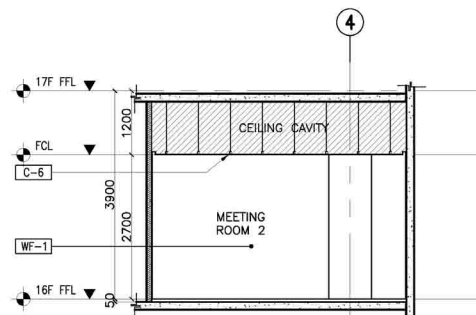
11 16F LPSD & FSD MEETING ROOM 2 SECTION THRU "C" A-910F SCALE: 1:50M
