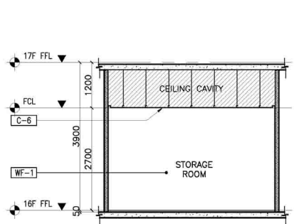
1 16F LPSD & FSD STORAGE ROOM (RIGHT) SECTION THRU "A" A-910F SCALE: 1:50M
