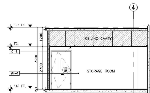
7 16F LPSD & FSD STORAGE ROOM (LEFT) SECTION THRU "C" A-910F SCALE: 1:50M
