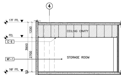
5 16F LPSD & FSD STORAGE ROOM (LEFT) SECTION THRU "A" A-910F SCALE: 1:50M
