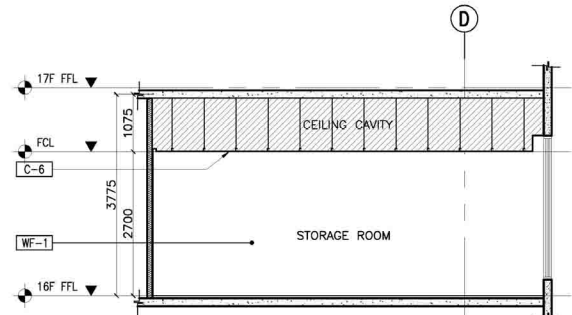
4 16F LPSD & FSD STORAGE ROOM (RIGHT) SECTION THRU "D" A-910F SCALE: 1:50M
