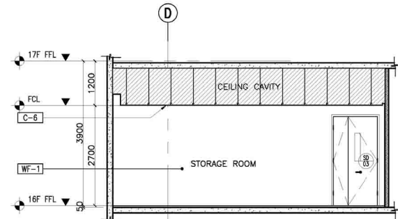
2 16F LPSD & FSD STORAGE ROOM (RIGHT) SECTION THRU "B" A-910F SCALE: 1:50M
