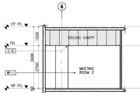
9 16F LPSD & FSD MEETING ROOM 2 SECTION THRU "A" A-910F SCALE: 1:50M
