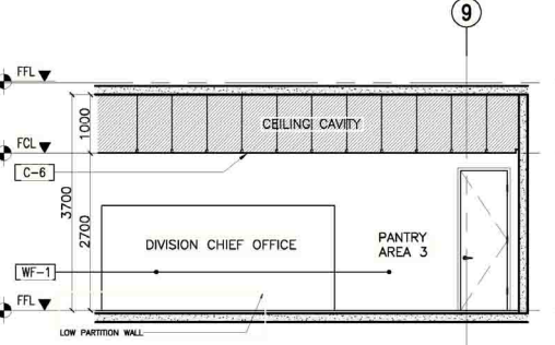
15 12F RECEIVING AREA SECTION THRU "A" A-907E SCALE: 1:50M
