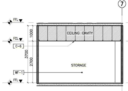
8 12F STORAGE AREA SECTION THRU "A" A-907E SCALE: 1:50M
