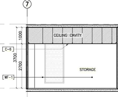
10 12F STORAGE AREA SECTION THRU "C" A-907E SCALE: 1:50M
