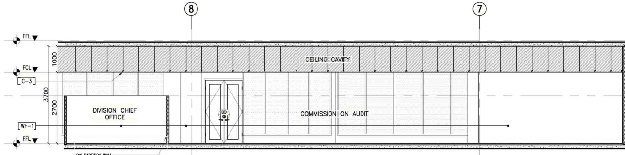
2 12F COMMISSION ON AUDIT SECTION THRU "C" A-907E SCALE: 1:50M
