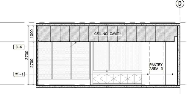
18 12F RECEIVING AREA SECTION THRU "C" A-907E SCALE: 1:50M
