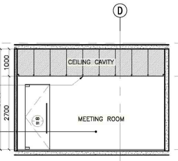
7 12F MEETING ROOM SECTION THRU "D" A-907E SCALE: 1:50M
