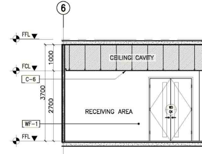
12 12F RECEIVING AREA SECTION THRU "A" A-907E SCALE: 1:50M
