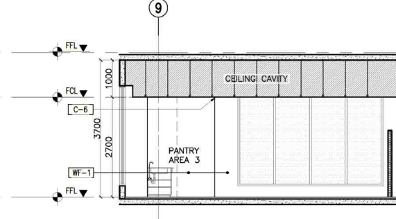
17 12F RECEIVING AREA SECTION THRU "C" A-907E SCALE: 1:50M
