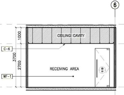
13 12F RECEIVING AREA SECTION THRU "B" A-907E SCALE: 1:50M
