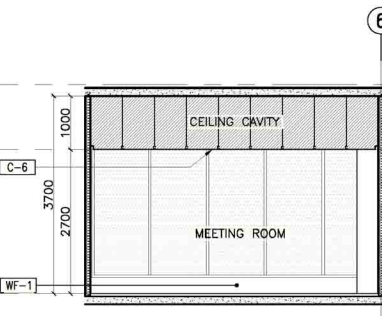
6 12F MEETING ROOM SECTION THRU "C" A-907E SCALE: 1:50M
