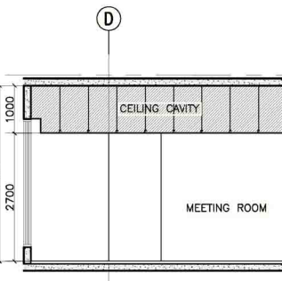
5 12F MEETING ROOM SECTION THRU "B" A-907E SCALE: 1:50M
