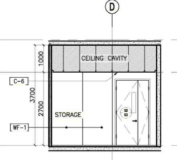
11 12F STORAGE AREA SECTION THRU "D" A-907E SCALE: 1:50M
