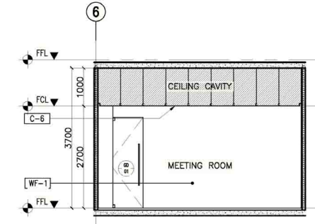
4 12F MEETING ROOM SECTION THRU "A" A-907E SCALE: 1:50M
