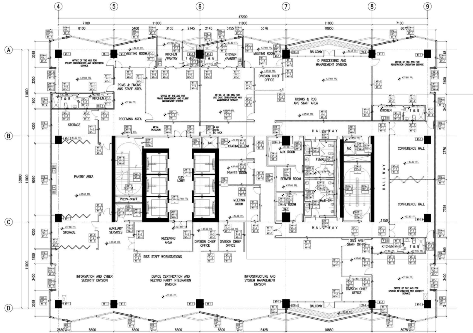
1 11TH FLOOR WALL SETTING-OUT PLAN A-612 SCALE 1:100 M.
