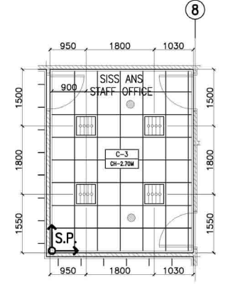
10 11F - SISS ANS STAFF OFFICE REFLECTED CEILING PLAN A-906G SCALE: 1:50M.
