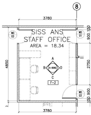
9 11F - SISS ANS STAFF OFFICE BLOW-UP PLAN A-906G SCALE: 1:50M.
