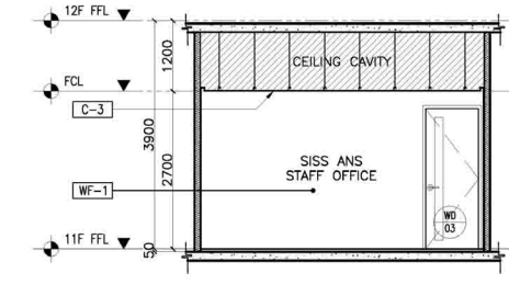
12 11F - SISS ANS STAFF OFFICE SECTION THRU "B" A-906G SCALE: 1:50M.
