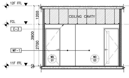
14 11F - SISS ANS STAFF OFFICE SECTION THRU "D" A-906G SCALE: 1:50M.
