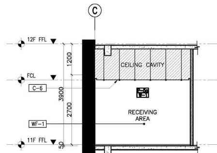
7 11F - SISS STAFF RECEIVING AREA SECTION THRU "D" A-906G SCALE: 1:50M.
