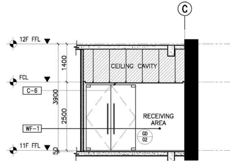
5 11F - SISS STAFF RECEIVING AREA SECTION THRU "B" A-906G SCALE: 1:50M.
