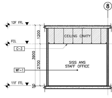
11 11F - SISS ANS STAFF OFFICE SECTION THRU "A" A-906G SCALE: 1:50M.
