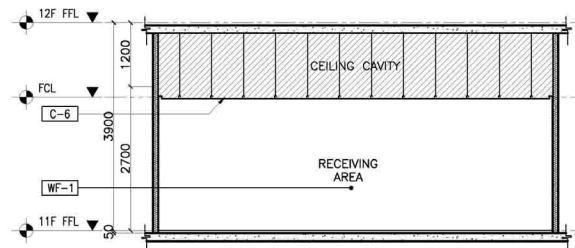
6 11F - SISS STAFF RECEIVING AREA SECTION THRU "C" A-906G SCALE: 1:50M.
