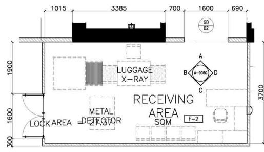
2 11F - SISS STAFF RECEIVING AREA BLOW-UP PLAN A-906G SCALE: 1:50M.
