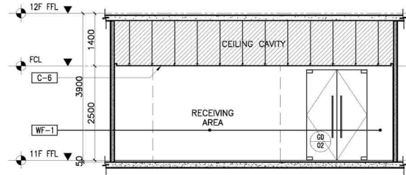
4 11F - SISS STAFF RECEIVING AREA SECTION THRU "A" A-906G SCALE: 1:50M.
