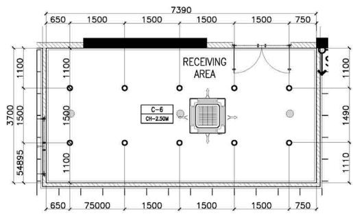
3 11F - SISS STAFF RECEIVING AREA REFLECTED CEILING PLAN A-906G SCALE: 1:50M.
