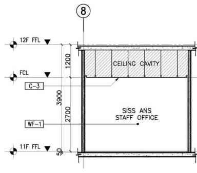
13 11F - SISS ANS STAFF OFFICE SECTION THRU "C" A-906G SCALE: 1:50M.
